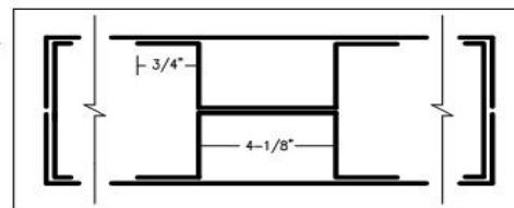
TOP VIEW OF SINGLE STIFFENER
