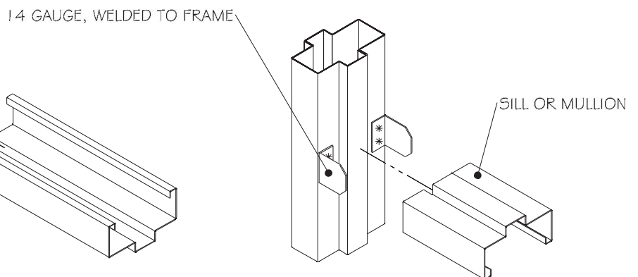
NON-LABELED MID-MULLION SPLICE
