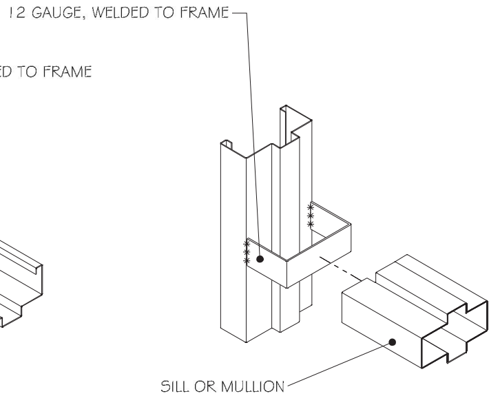
LABELED MID-MULLION SPLICE
