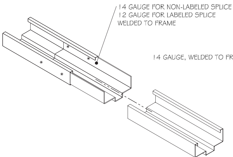
HEADER OR SILL SPLICE
