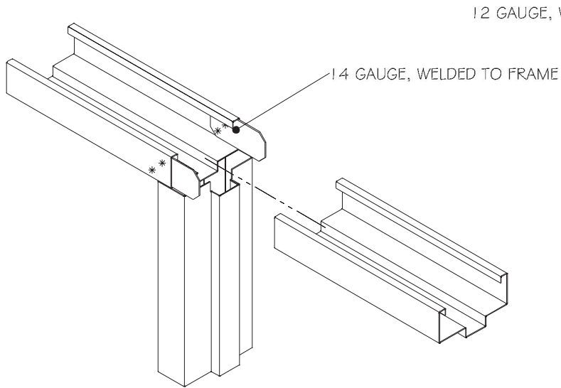
NON-LABELED HEADER SPLICE
